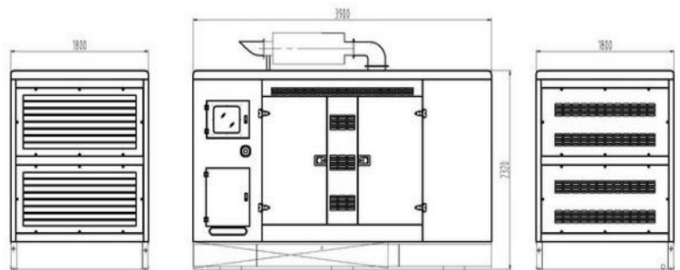
Soundproof Type Overall size: 3700 × 1700 × 2100mm(L*W*H) Weight: 4550kg
