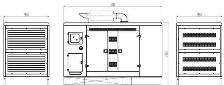
Soundproof Type Overall size: 3700×1700×2100mm(L*W*H) Weight: 4550kg
