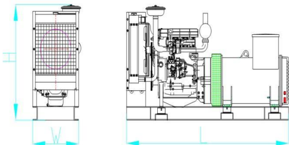
Open Type (Standard Configuration) Overall Size: 3150×1270 ×2100mm(L*W*H) Weight: 3600kg
