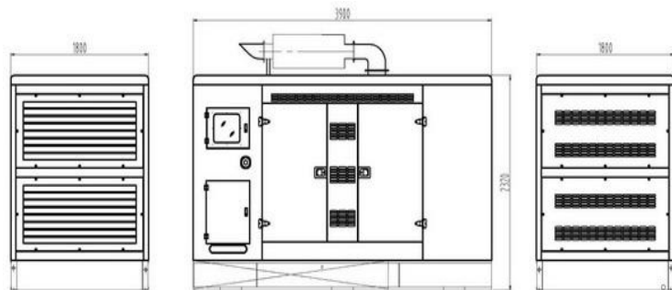
Soundproof Type Overall size: 3600× 1700×2100mm(L*W*H) Weight: 3350kg
