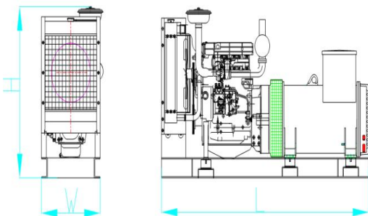
Open Type (Standard Configuration) Overall Size: 3000×1270 ×2040mm(L*W*H) Weight: 2500kg
