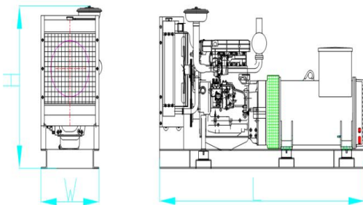
Open Type (Standard Configuration) Overall Size: 2980×1110 ×1650mm(L*W*H) Weight: 2200kg
