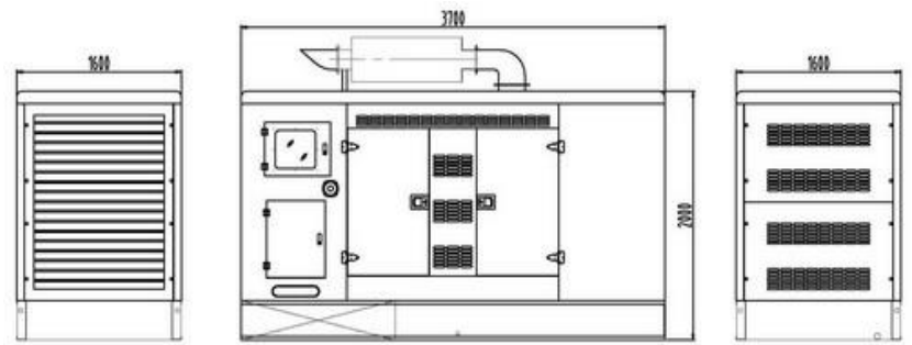
Soundproof Type Overall size: 3700× 1600×2180mm(L*W*H) Weight: 4000kg
